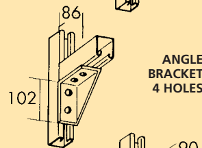
WIDE TEE ANGLE BRACKET 4 HOLES
