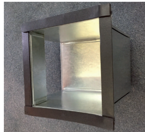
1. Lay in gasket across bolt holes x 4 flanges
