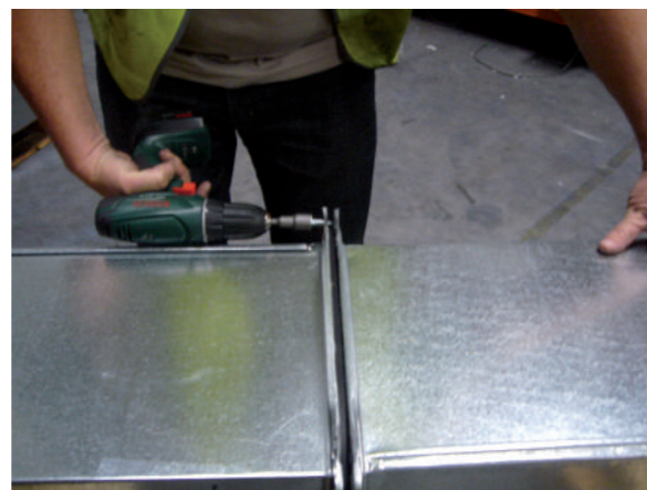
2. Screw in QuikScrews™ through the gasket into each of the QuikCorners*™ x 4 (NO NEED TO ALIGN BOLT HOLES)
