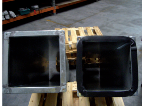
1. Lay in gasket x 4 flanges
