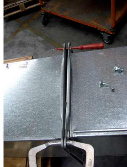
2. Align bolt holes with screwdriver or corner alignment
